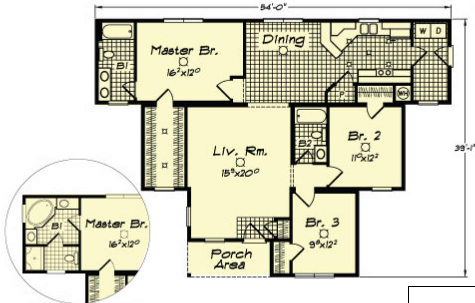
OPTIONAL BATH 57'-4" REAR MODULE LENGTH HOUSE = 1537 SQ FT WITH OPTIONAL BATH
